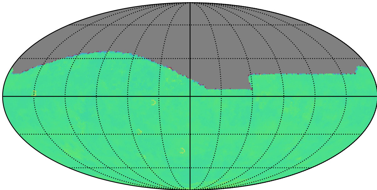
ddf_loaded_half_fl8_v3.3_10yrs r: Kuiper rotTelPos
