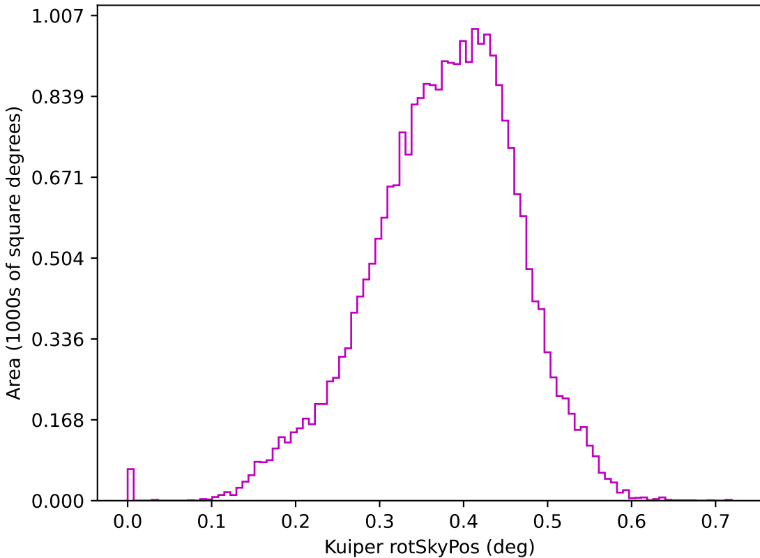
ddf_loaded_half_fl8_v3.3_10yrs z: Kuiper rotSkyPos
