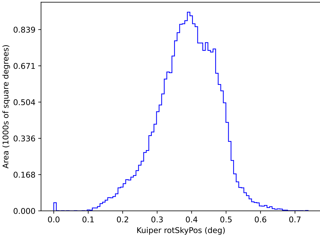
ddf_loaded_half_fl8_v3.3_10yrs y: Kuiper rotSkyPos
