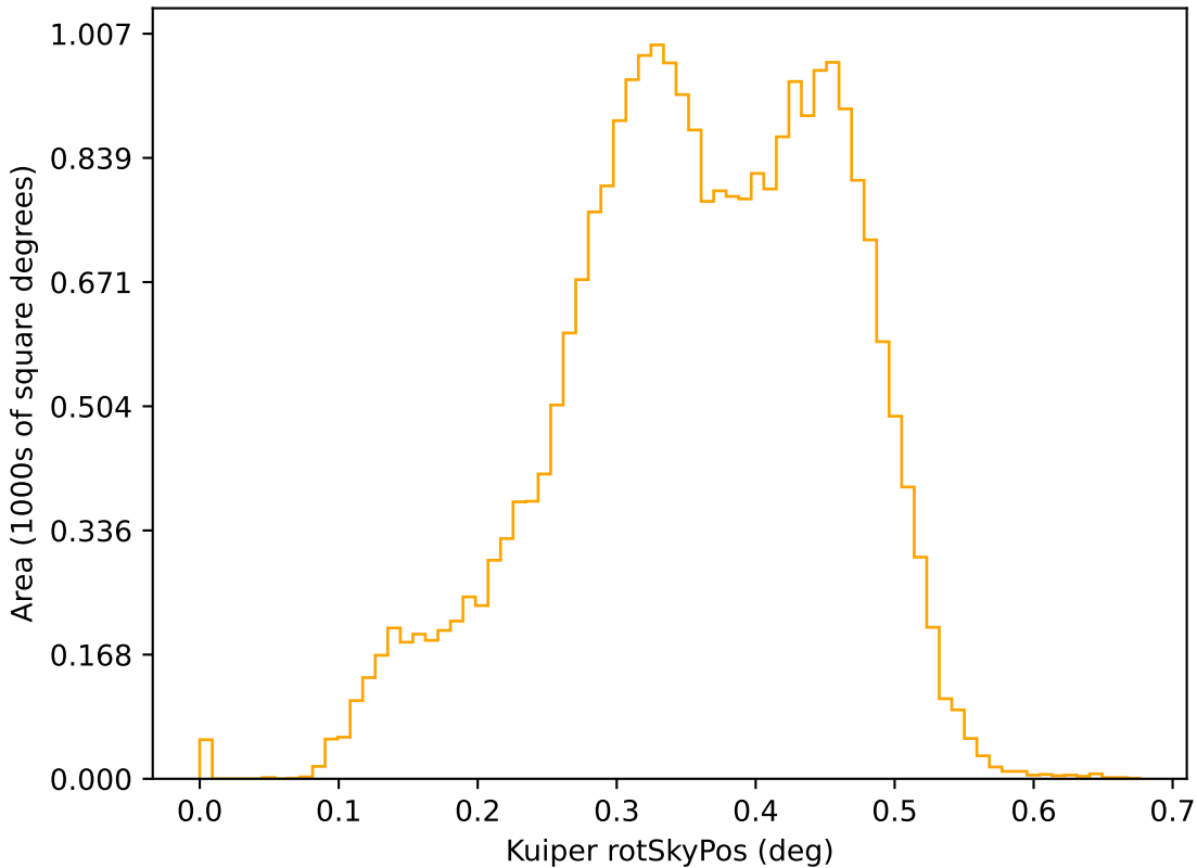
ddf_loaded_half_fl8_v3.3_10yrs r: Kuiper rotSkyPos
