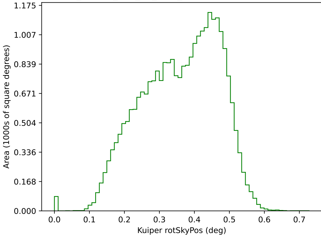
ddf_loaded_half_fl8_v3.3_10yrs g: Kuiper rotSkyPos
