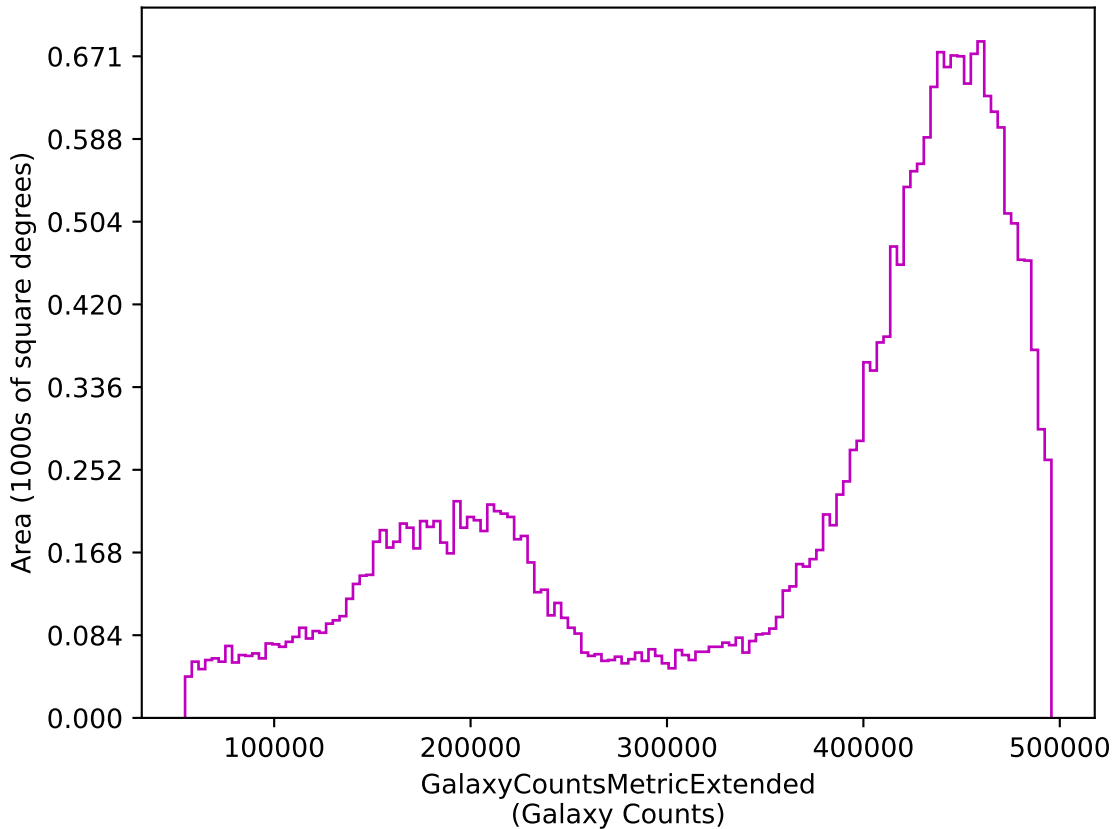
ddf_loaded_half_fl8_v3.3_10yrs z: GalaxyCountsMetricExtended
