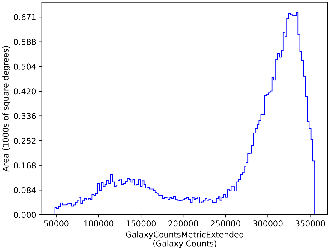
ddf_loaded_half_fl8_v3.3_10yrs y: GalaxyCountsMetricExtended
