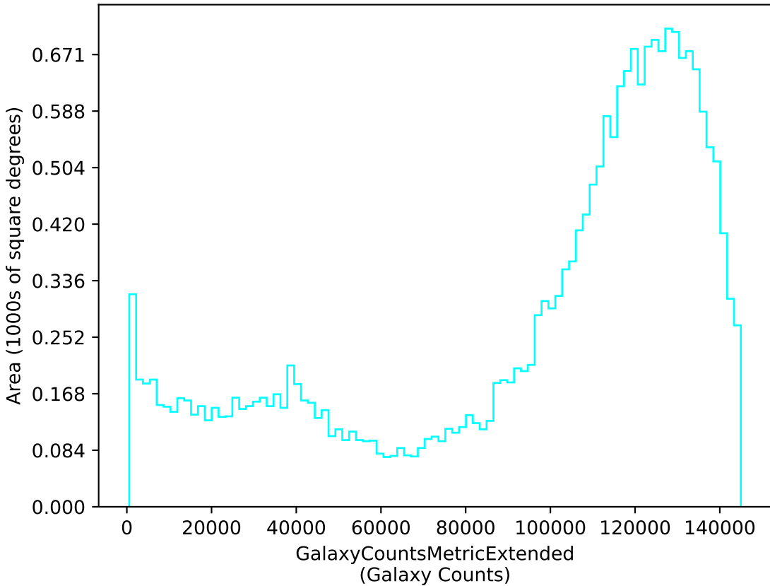
ddf_loaded_half_fl8_v3.3_10yrs u: GalaxyCountsMetricExtended
