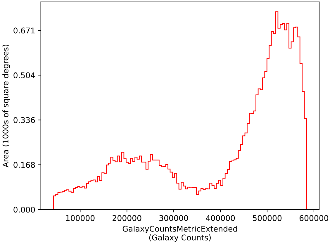
ddf_loaded_half_fl8_v3.3_10yrs i: GalaxyCountsMetricExtended
