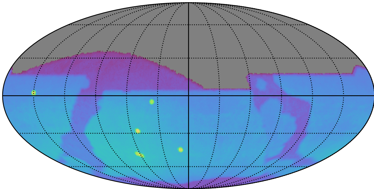
ddf_loaded_half_fl8_v3.3_10yrs : Brown Dwarf, L7
