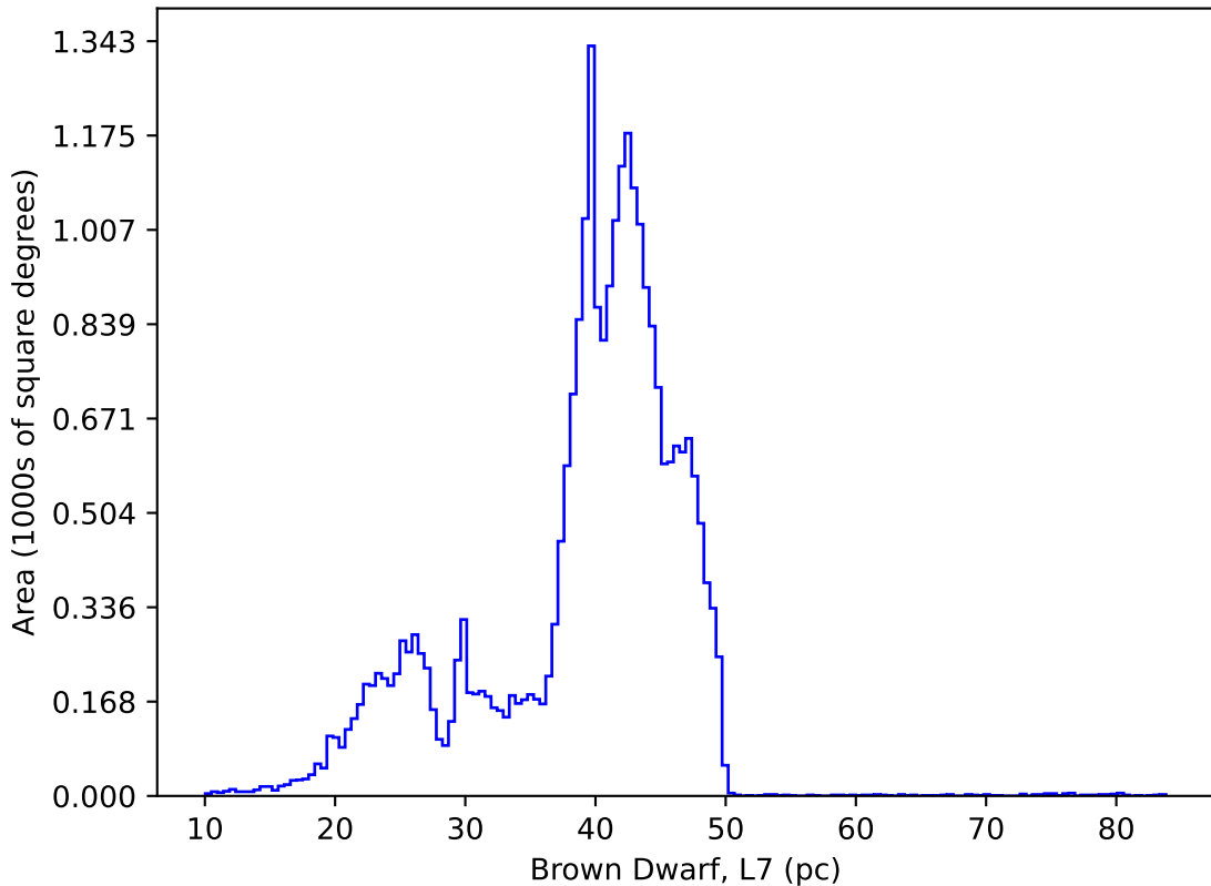
ddf_loaded_half_fl8_v3.3_10yrs : Brown Dwarf, L7
