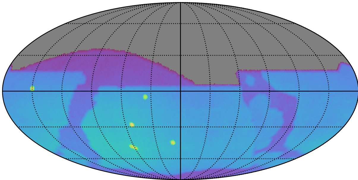
ddf_loaded_half_fl8_v3.3_10yrs : Brown Dwarf, L4
