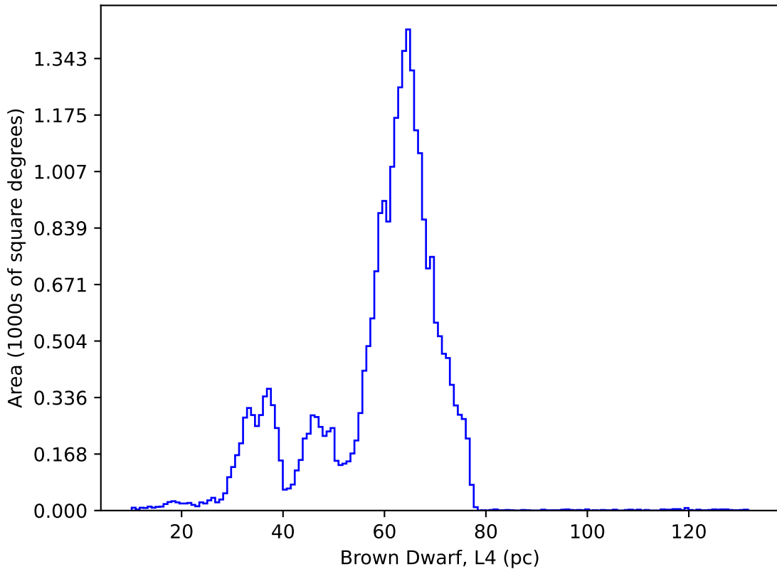
ddf_loaded_half_fl8_v3.3_10yrs : Brown Dwarf, L4
