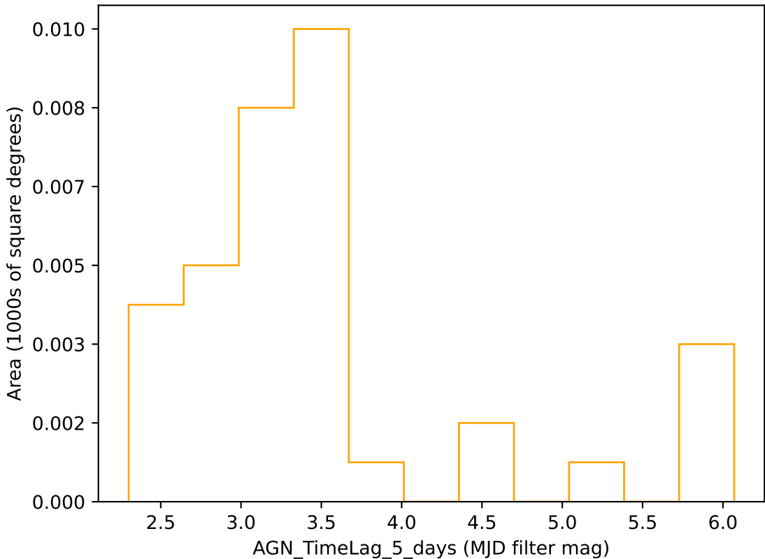
ddf_loaded_half_fl8_v3.3_10yrs r band: AGN_TimeLag_5_days
