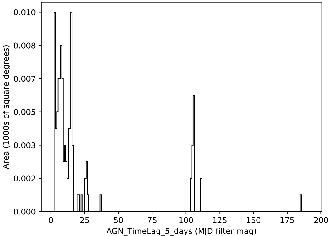
ddf_loaded_half_fl8_v3.3_10yrs all bands: AGN_TimeLag_5_days
