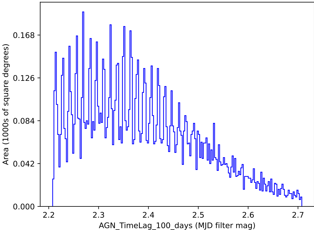
ddf_loaded_half_fl8_v3.3_10yrs y band: AGN_TimeLag_100_days
