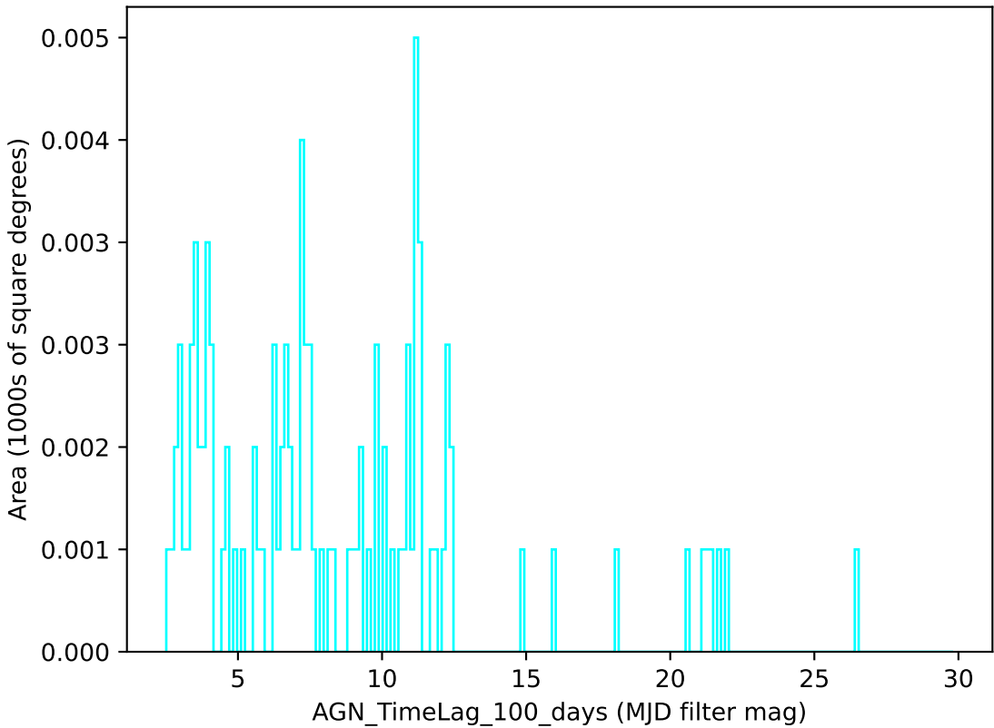
ddf_loaded_half_fl8_v3.3_10yrs u band: AGN_TimeLag_100_days
