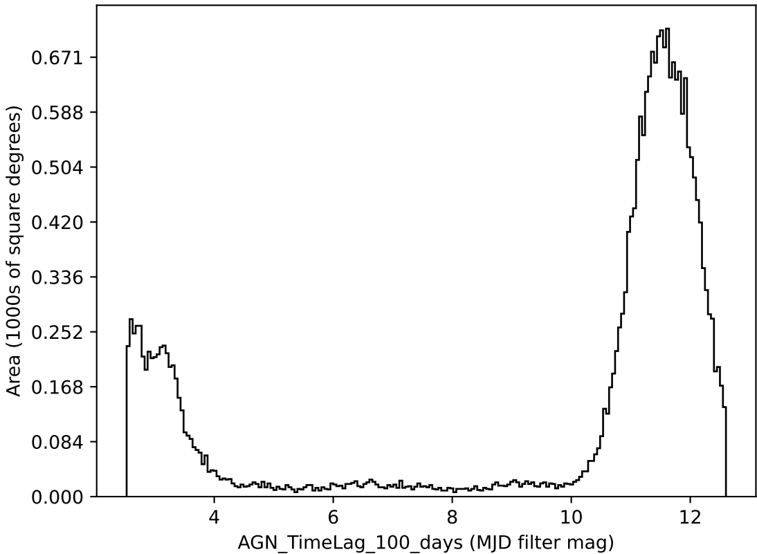
ddf_loaded_half_fl8_v3.3_10yrs all bands: AGN_TimeLag_100_days
