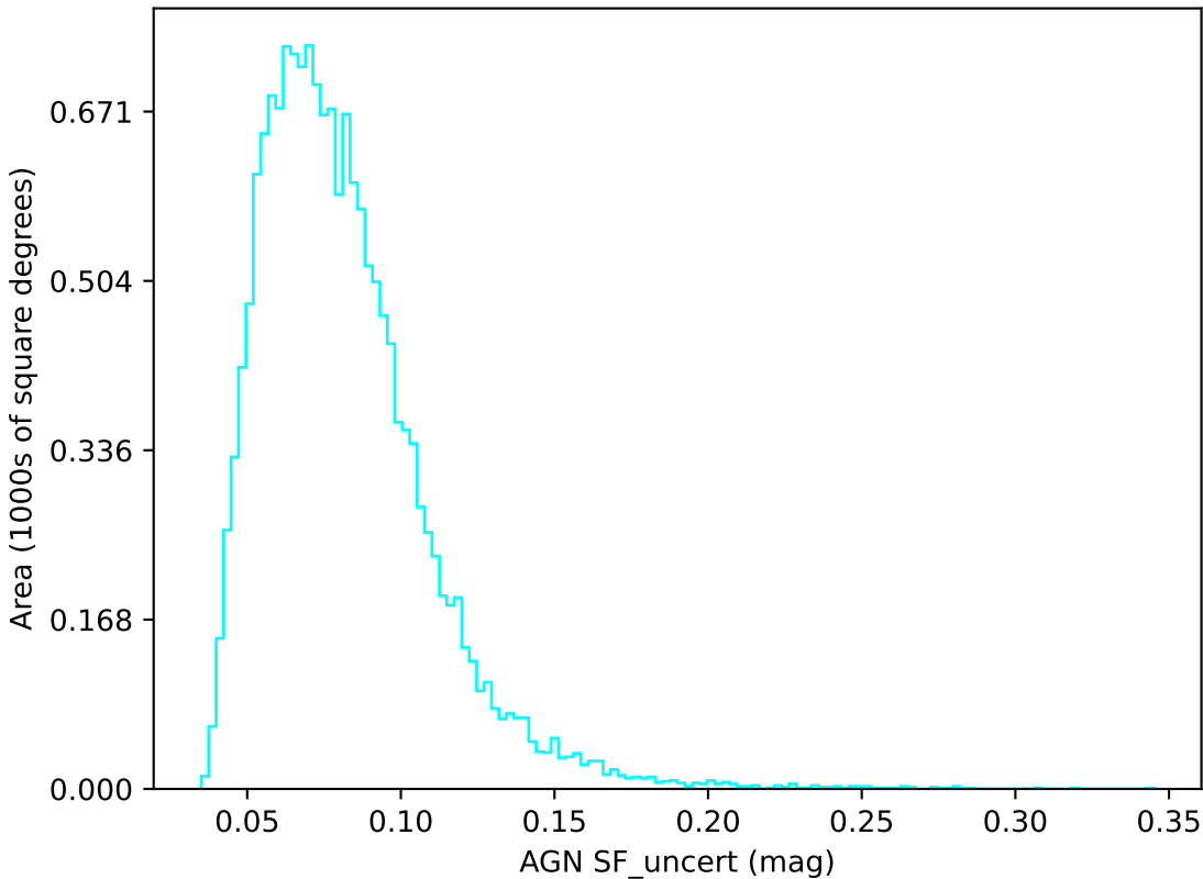
ddf_loaded_half_fl8_v3.3_10yrs u band: AGN SF_uncert
