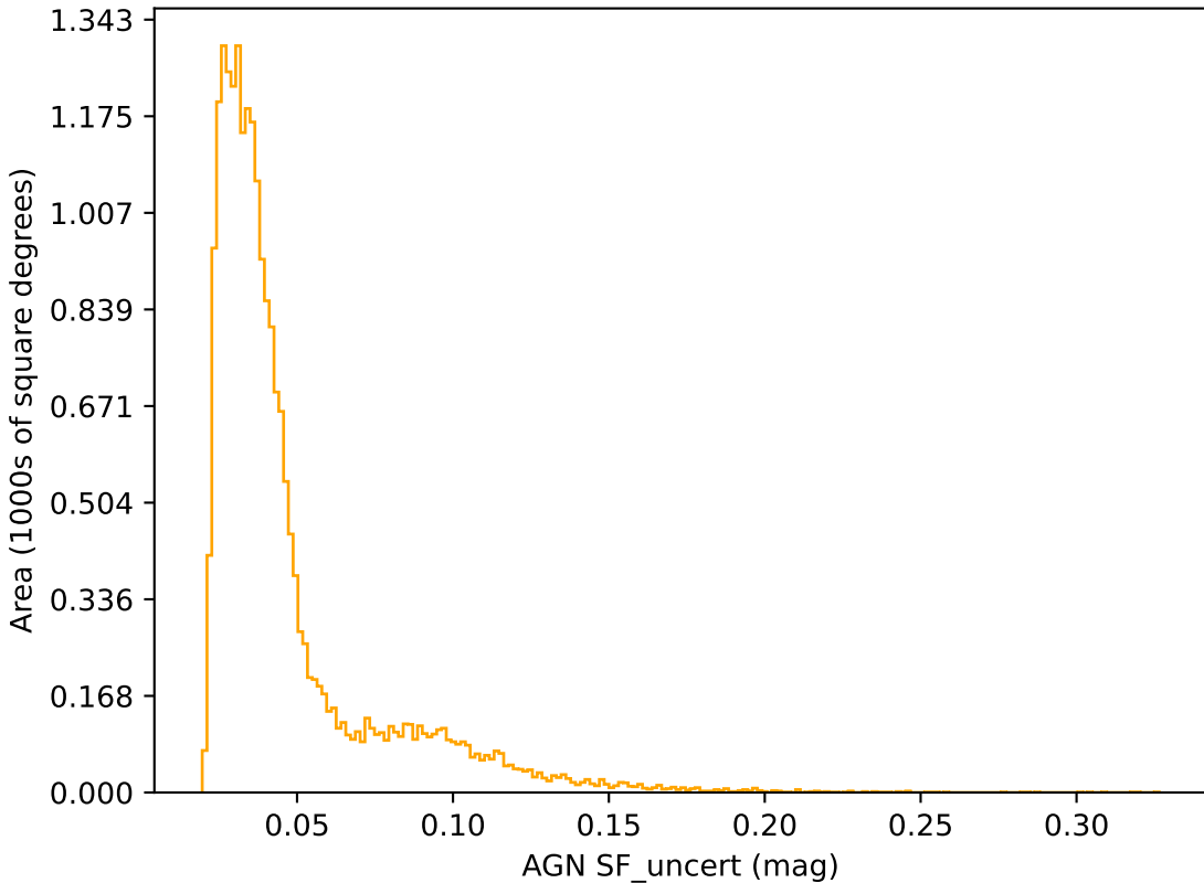
ddf_loaded_half_fl8_v3.3_10yrs r band: AGN SF_uncert
