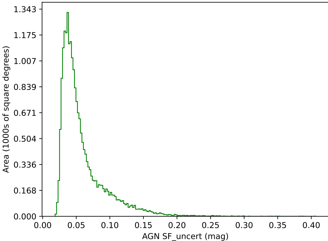
ddf_loaded_half_fl8_v3.3_10yrs g band: AGN SF_uncert
