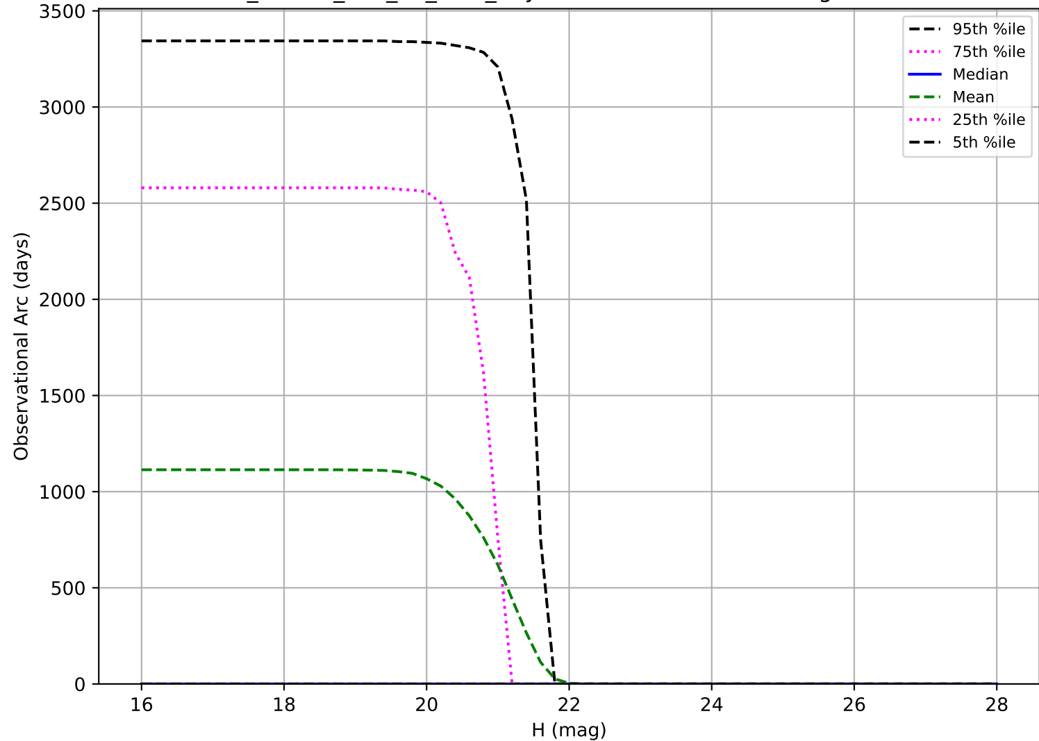
ddf_loaded_half_fl4_v3.4_10yrs: Observational Arc Length Vatira
