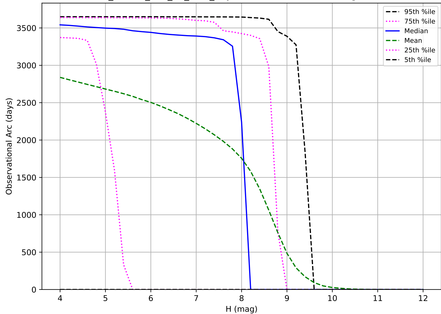
ddf_loaded_half_fl4_v3.4_10yrs: Observational Arc Length TNO
