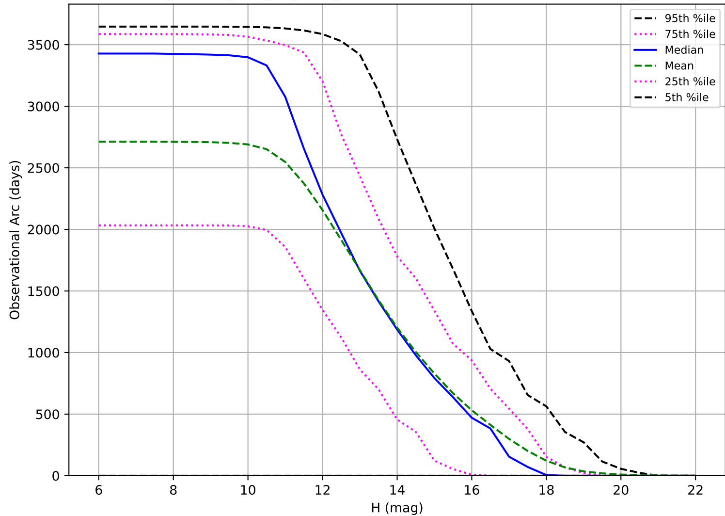
ddf_loaded_half_fl4_v3.4_10yrs: Observational Arc Length OCC_r5
