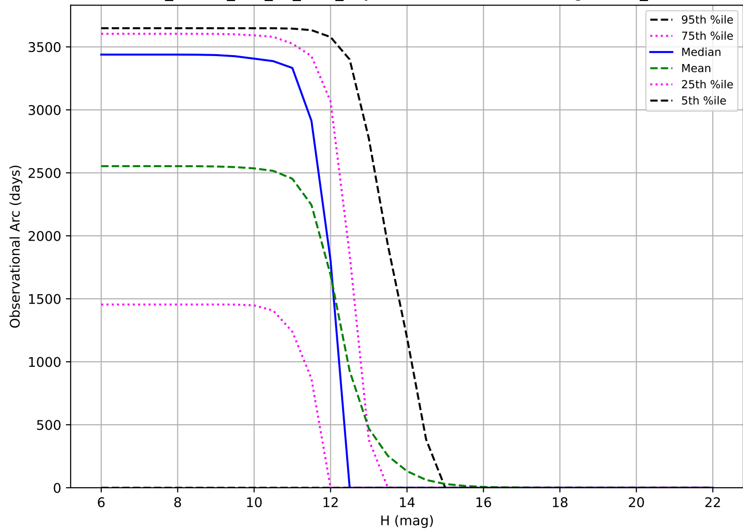
ddf_loaded_half_fl4_v3.4_10yrs: Observational Arc Length OCC_r20
