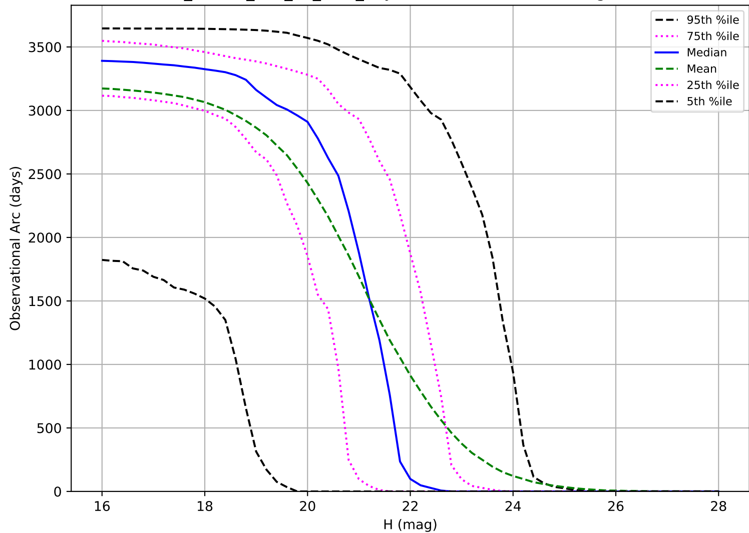
ddf_loaded_half_fl4_v3.4_10yrs: Observational Arc Length NEO
