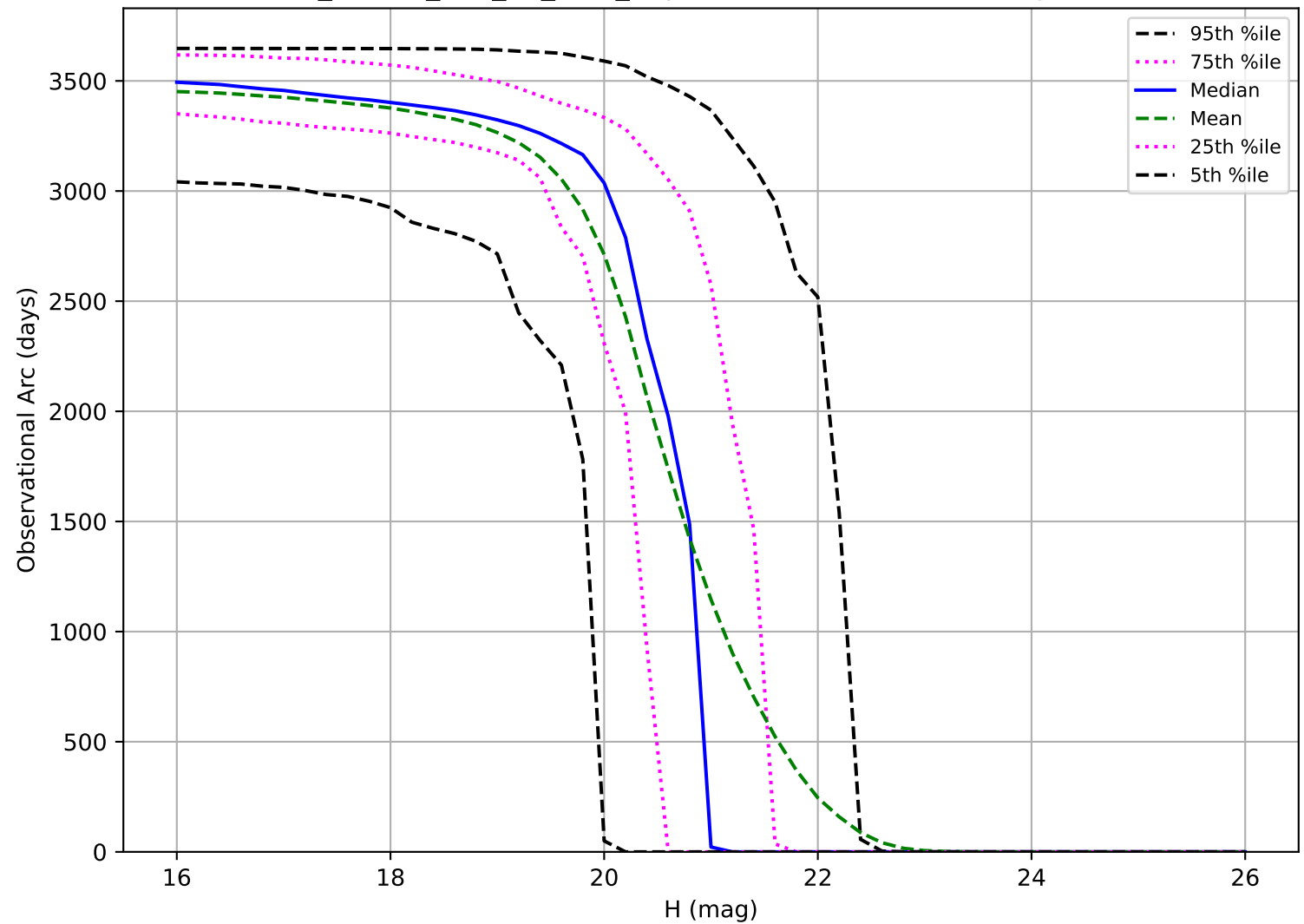
ddf_loaded_half_fl4_v3.4_10yrs: Observational Arc Length MBA
