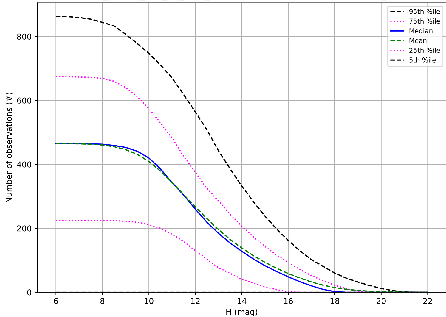
ddf_loaded_half_fl4_v3.4_10yrs: Number of observations OCC_r5
