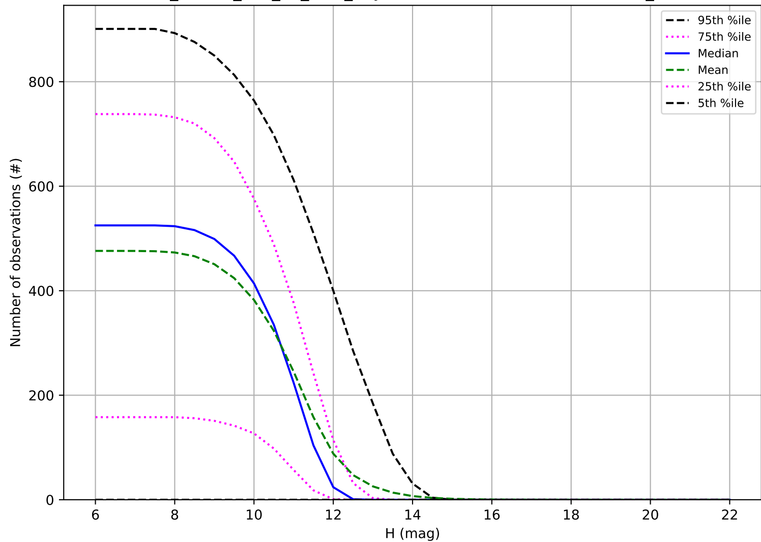
ddf_loaded_half_fl4_v3.4_10yrs: Number of observations OCC_r20
