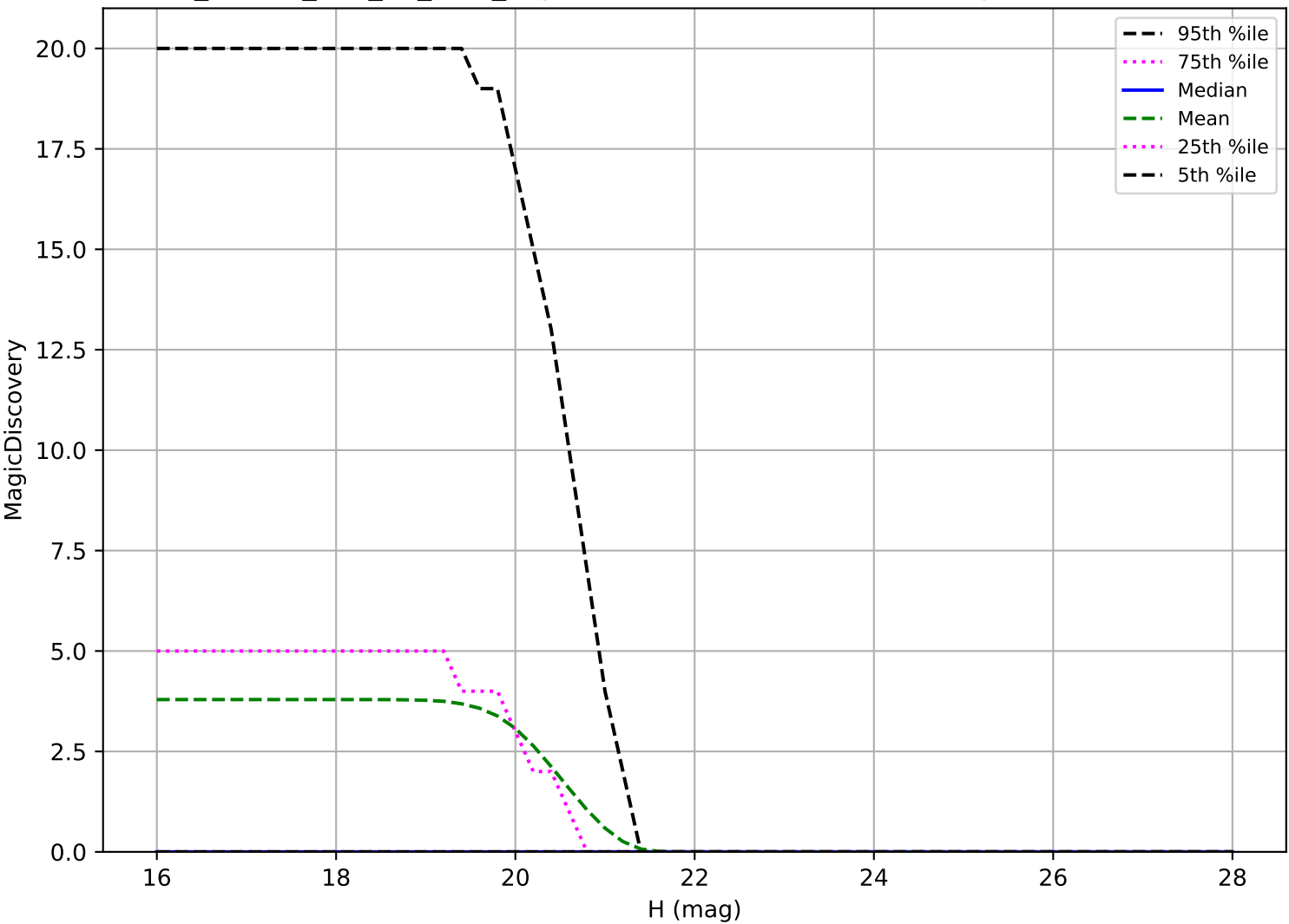
ddf_loaded_half_fl4_v3.4_10yrs: Vatira 6 detections in 60 nights detection loss
