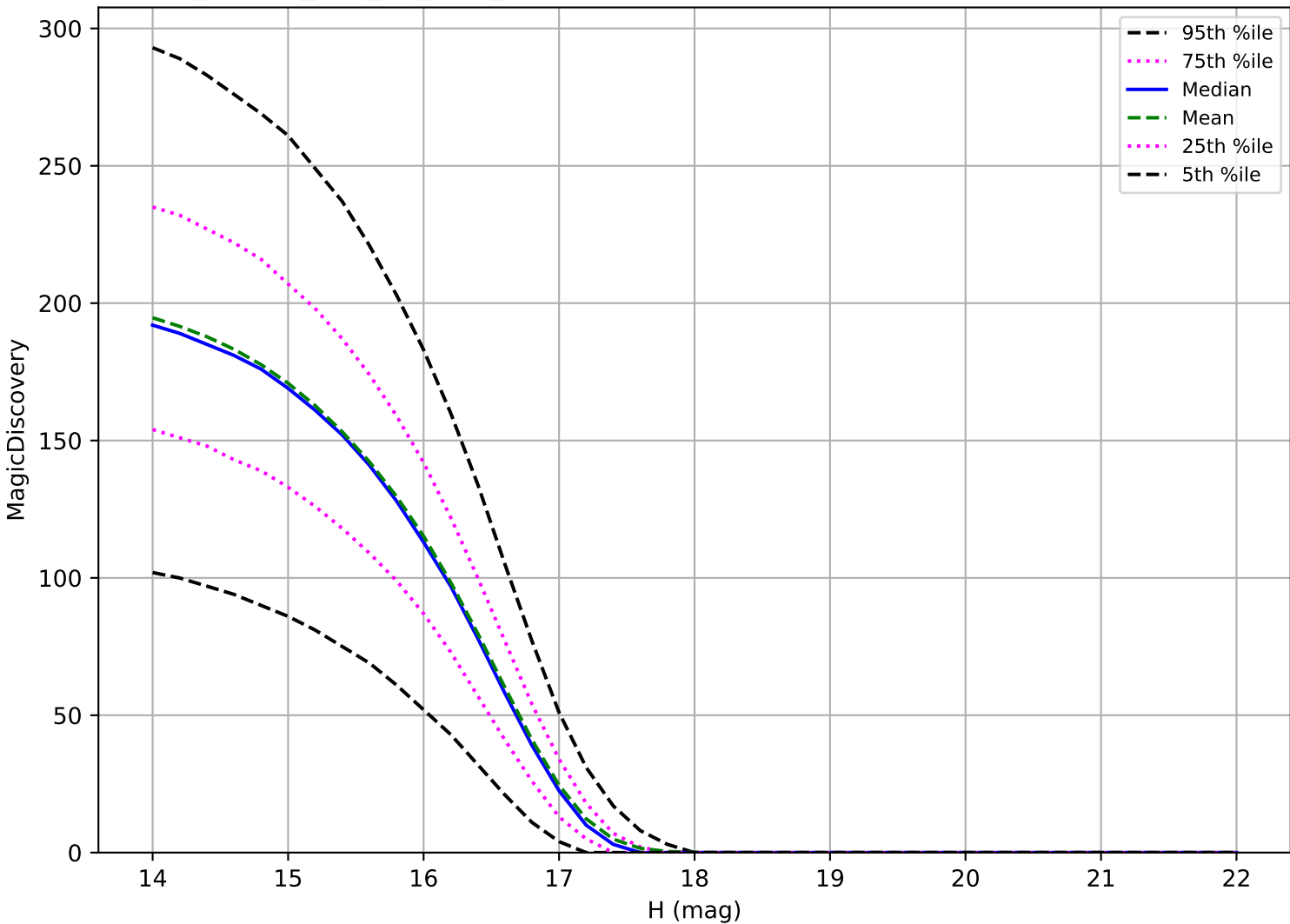
ddf_loaded_half_fl4_v3.4_10yrs: Trojan 6 detections in 60 nights detection loss
