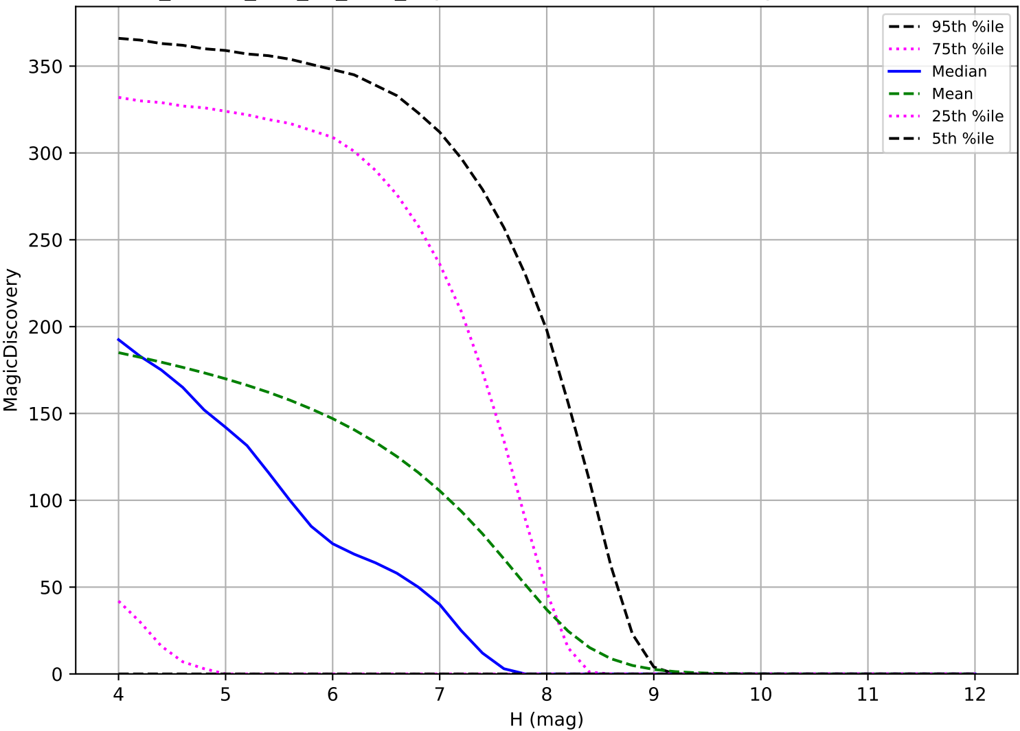
ddf_loaded_half_f14_v3.4_10yrs: TNO 6 detections in 60 nights detection loss
