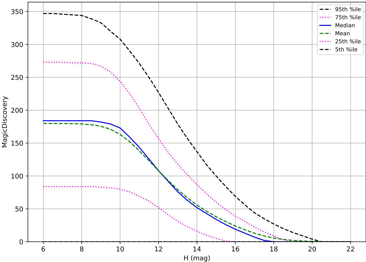
ddf_loaded_half_fl4_v3.4_10yrs: OCC_r5 6 detections in 60 nights detection loss
