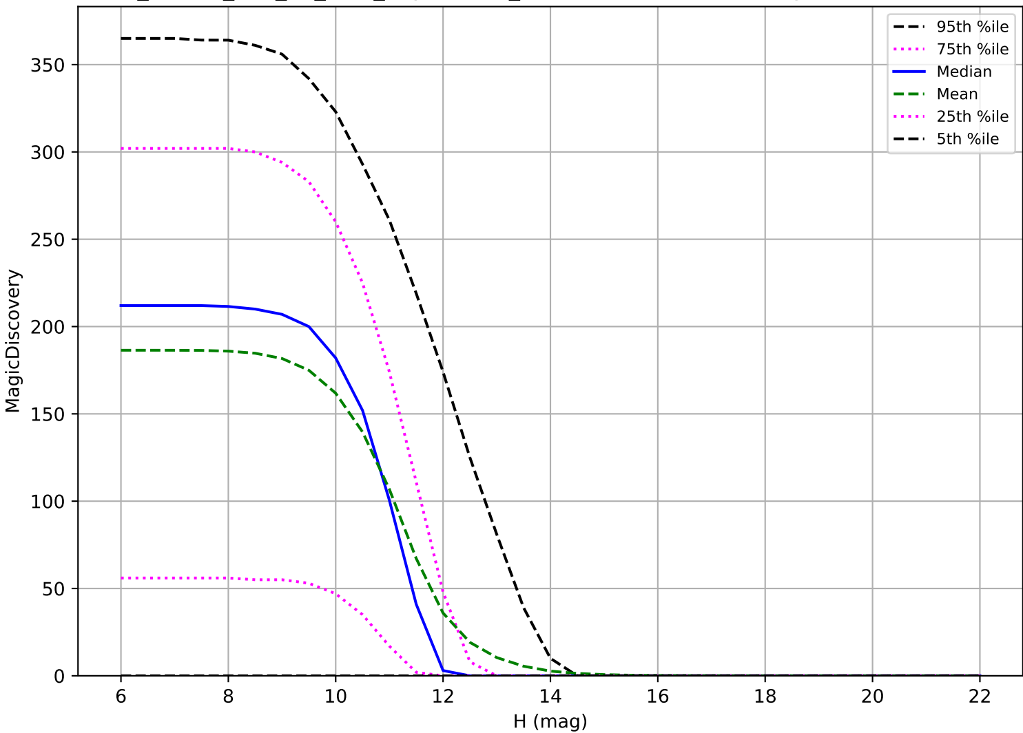
ddf_loaded_half_fl4_v3.4_10yrs: OCC_r20 6 detections in 60 nights detection loss
