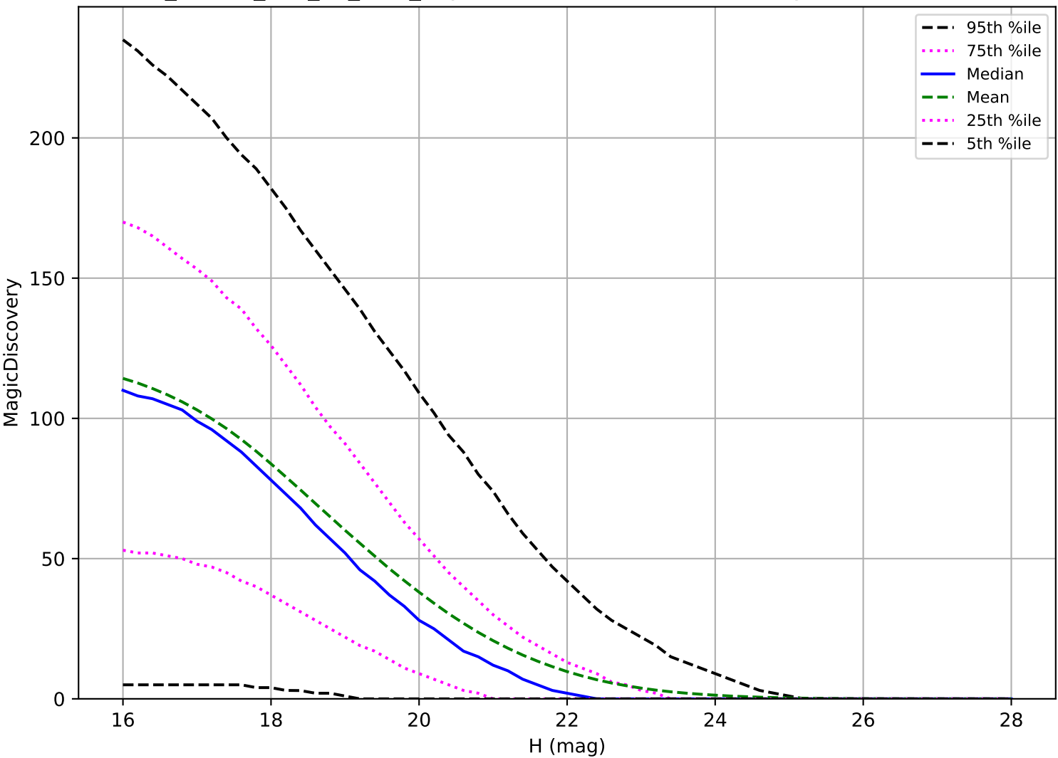
ddf_loaded_half_f14_v3.4_10yrs: NEO 6 detections in 60 nights detection loss
