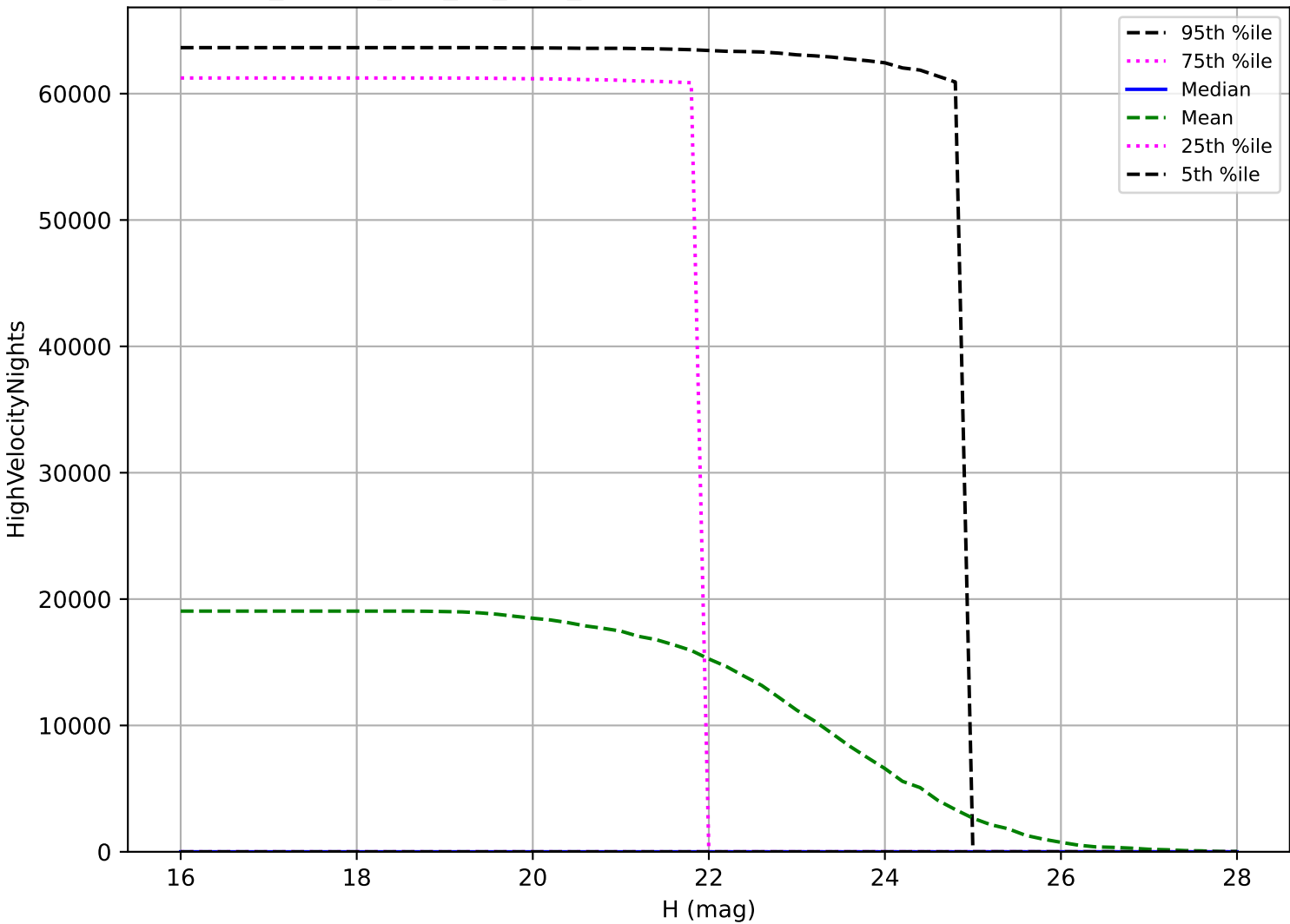
ddf_loaded_half_fl4_v3.4_10yrs: NEO High velocity pair detection loss
