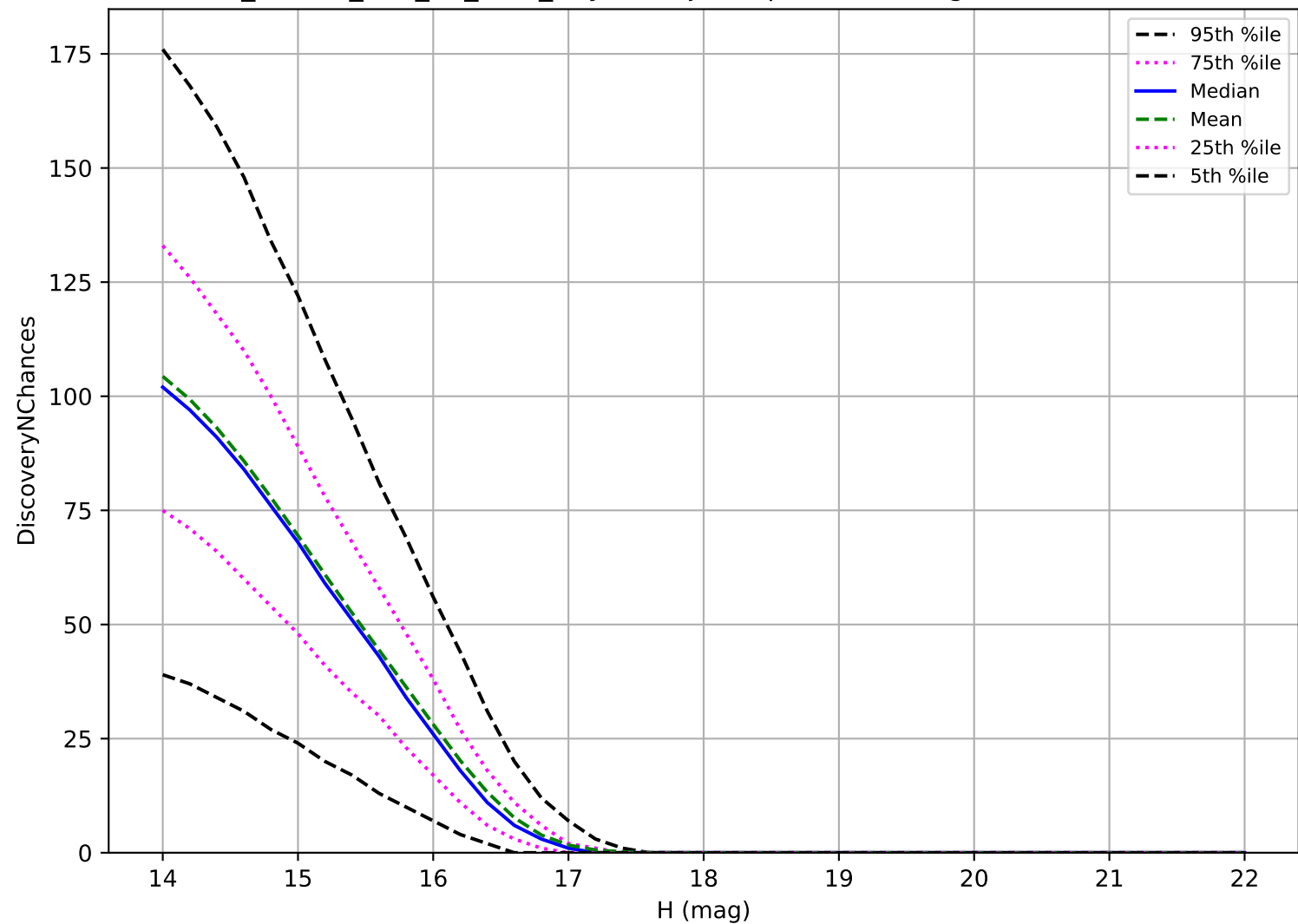
ddf_loaded_half_fl4_v3.4_10yrs: Trojan 3 pairs in 15 nights detection loss
