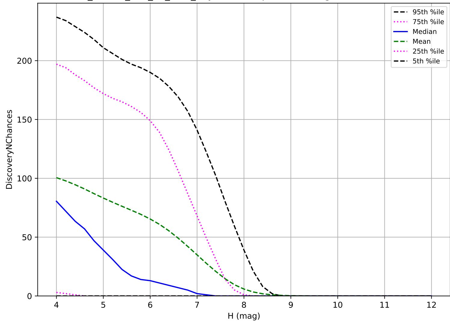
ddf_loaded_half_fl4_v3.4_10yrs: TNO 3 pairs in 15 nights detection loss
