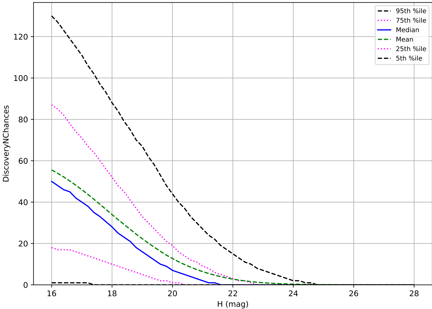
ddf_loaded_half_fl4_v3.4_10yrs: PHA 3 pairs in 15 nights detection loss
