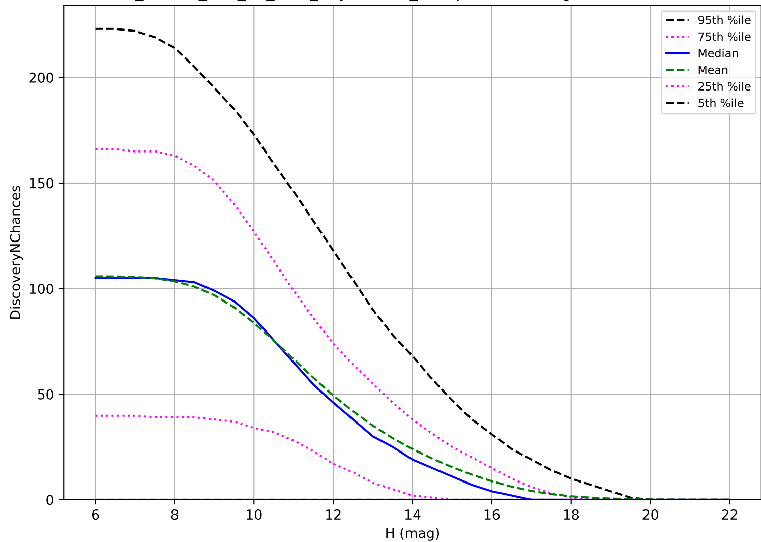
ddf_loaded_half_fl4_v3.4_10yrs: OCC_r5 3 pairs in 15 nights detection loss
