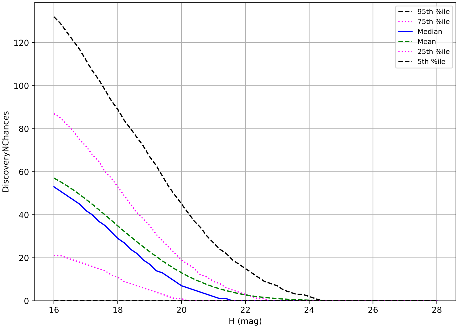
ddf_loaded_half_fl4_v3.4_10yrs: NEO 3 pairs in 15 nights detection loss
