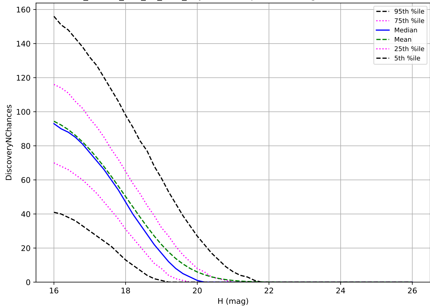
ddf_loaded_half_fl4_v3.4_10yrs: MBA 3 pairs in 15 nights detection loss
