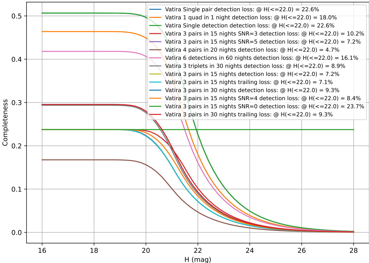
ddf_loaded_half_fl4_v3.4_10yrs: CumulativeCompleteness
