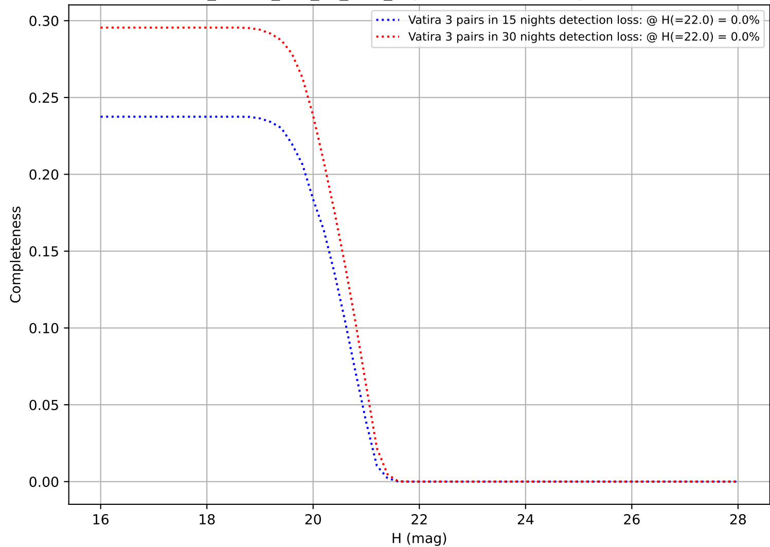
ddf_loaded_half_fl4_v3.4_10yrs: DifferentialCompleteness
