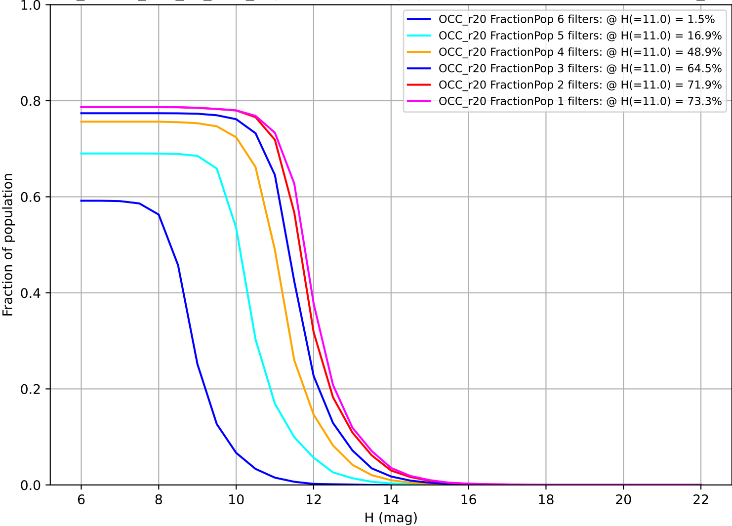
ddf_loaded_half_fl4_v3.4_10yrs: Fraction of population with colors in X filters OCC_r20
