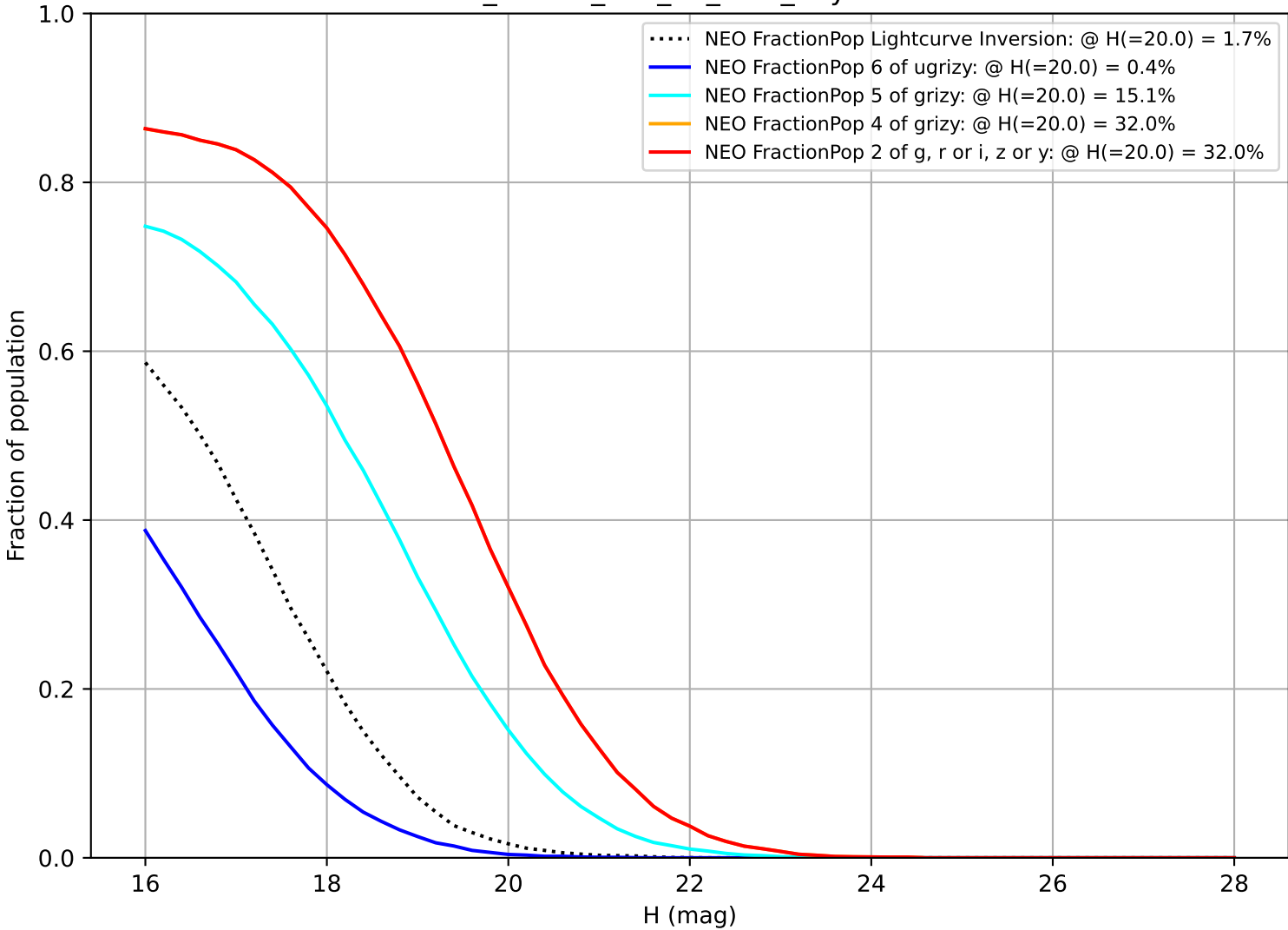
ddf_loaded_half_fl4_v3.4_10yrs NEO
