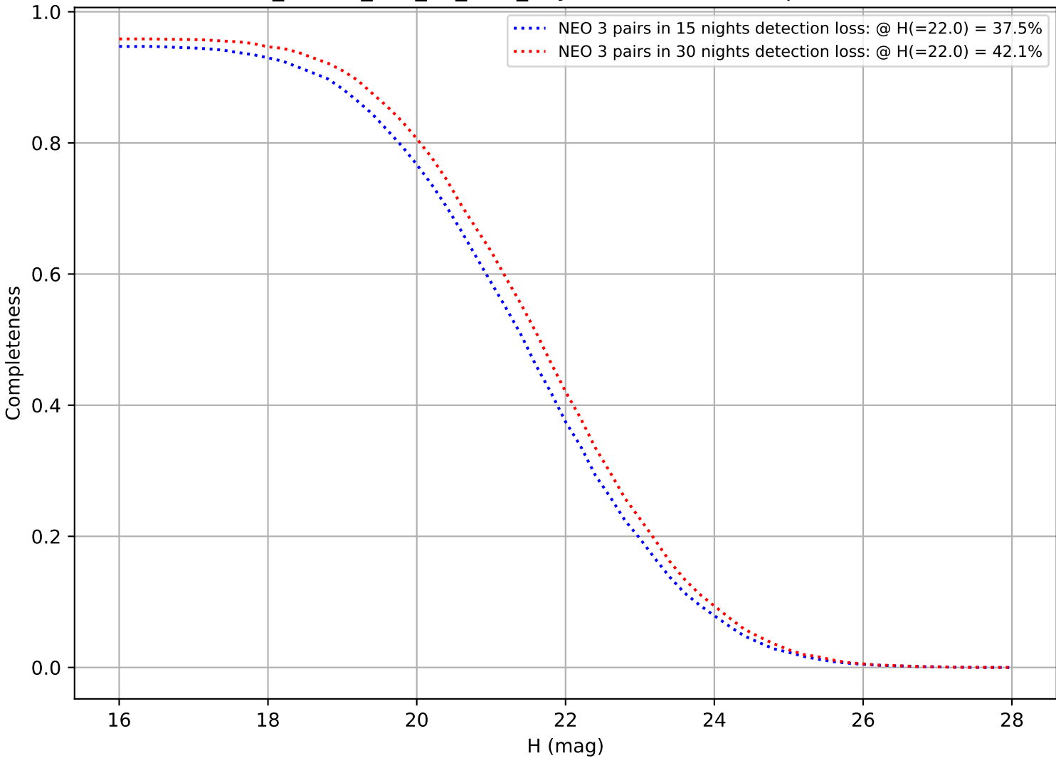
ddf_loaded_half_fl4_v3.4_10yrs: DifferentialCompleteness
