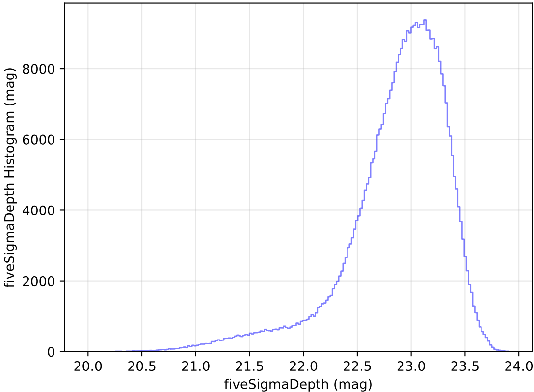
ddf_loaded_half_fl4_v3.4_10yrs z: fiveSigmaDepth Histogram
