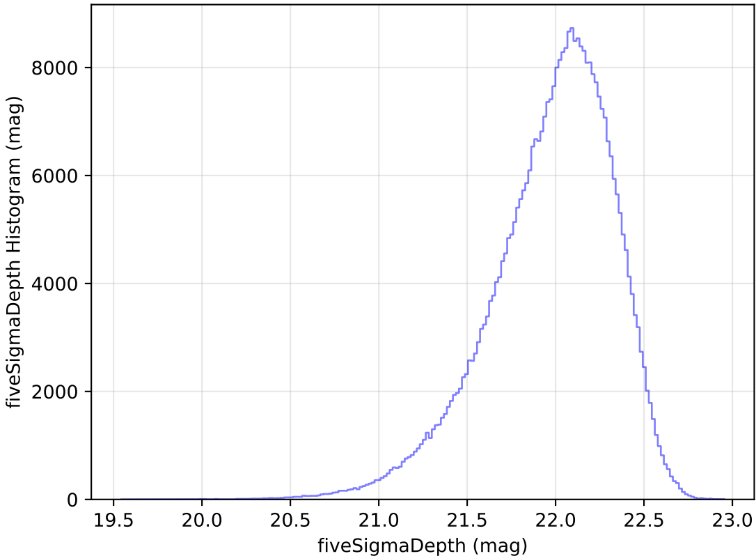
ddf_loaded_half_fl4_v3.4_10yrs y: fiveSigmaDepth Histogram
