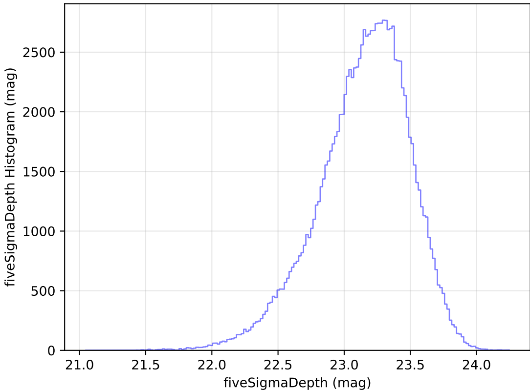
ddf_loaded_half_fl4_v3.4_10yrs u: fiveSigmaDepth Histogram
